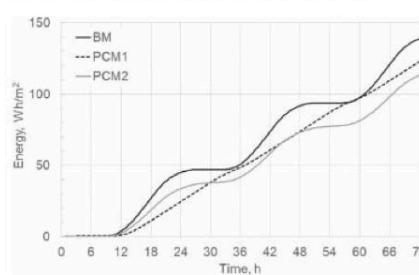
Figure 11. Time dependence of energy ( \text{Wh/m}^2 ) entering the room through the ceiling. Numerical integration of curves in Figure 10 for positive values of heat flux.
